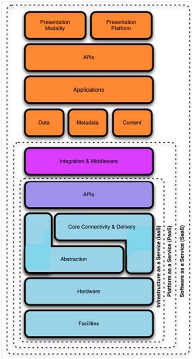
Figure 1) Cloud reference model (from Cloud Security Alliance Guidance Version 2.1 [2009]).
