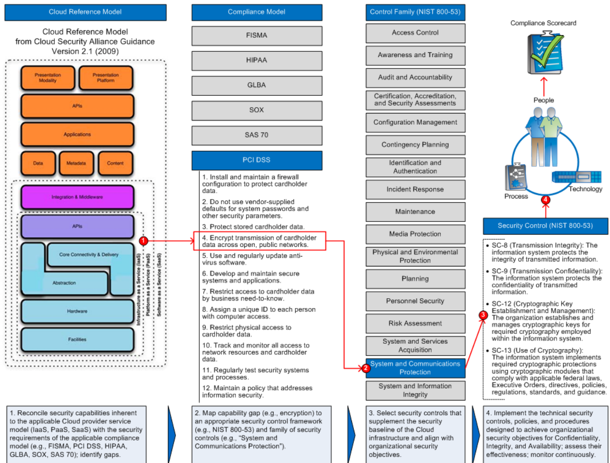
Figure 4) Mapping the cloud model to the security control and compliance model.
