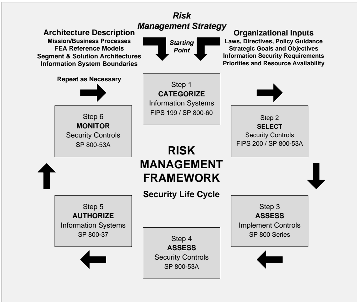
Figure 3) Risk management framework (from NIST Special Publication 800-37).
