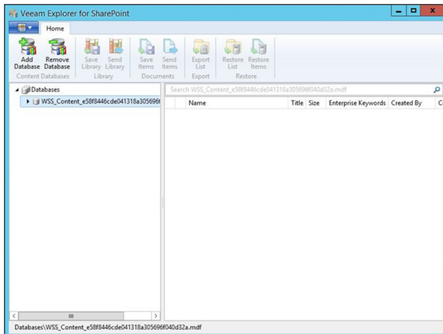
Figure 1 Interface
