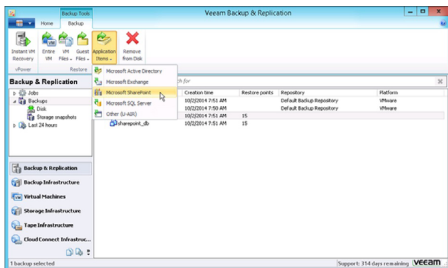
Figure 2 Interface
